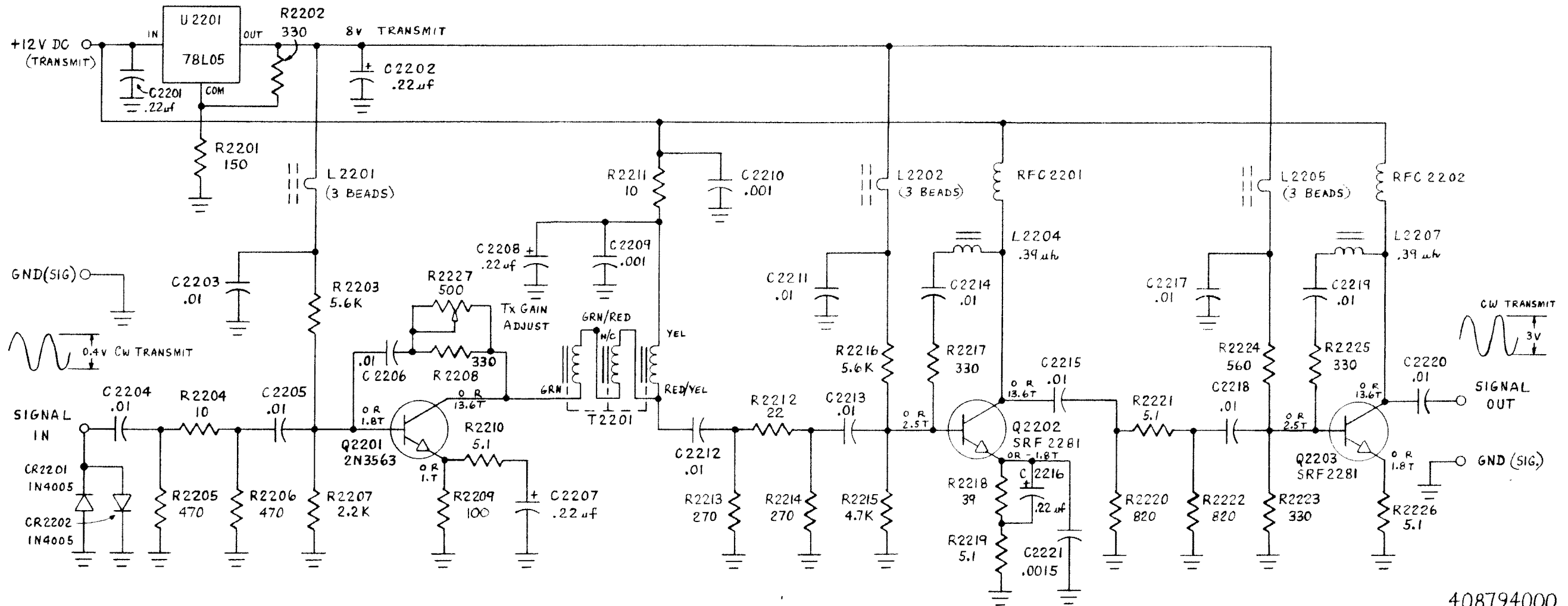
Fig. 2-37 Predriver P.A. Schematic
